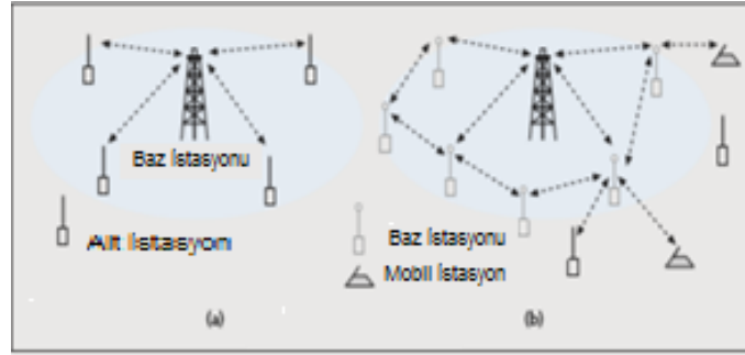
Şekil 1. (a) PMP Model (b) Örgü Model
