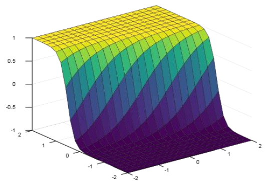
Figure 8: Regressive Soliton solutions of the equation (2) while wave speed c = 1 - 2\sqrt{2} .
