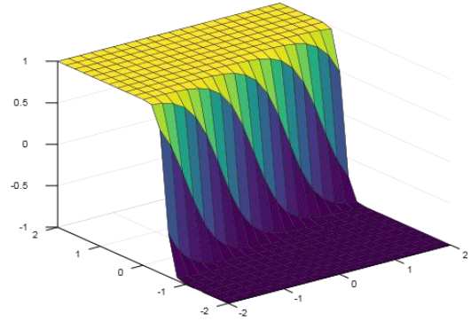
Figure 6: Soliton solutions of the equation (2) while wave speed c = 1 + 2\sqrt{2} .
