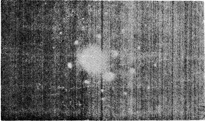
FIGURE 4. (a) Electron diffraction pattern taken from austenite-martensite interface,
