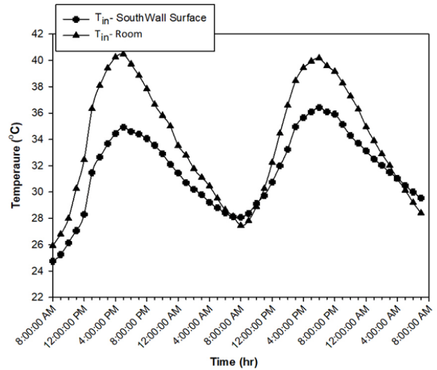
Figure 8. Temperature of the indoor and southern wall surfaces of room.
