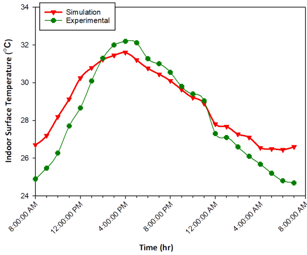
Figure 5. Verification of the interior temperature.
