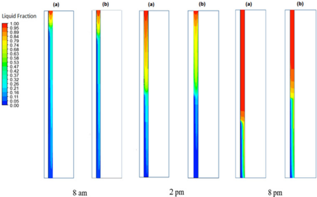
Figure 12. Liquid fraction contours of (a) Nano-enhanced PCM, (b) Pure PCM.
