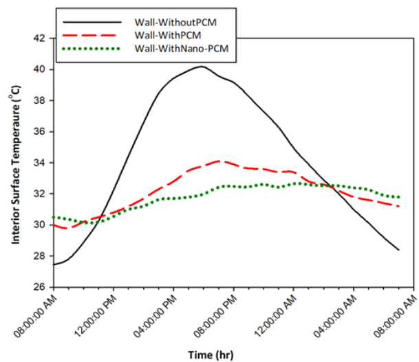
Figure 15. The interior surface temperature of the wall for PCM, Nano-enhanced PCM, and without PCM.
