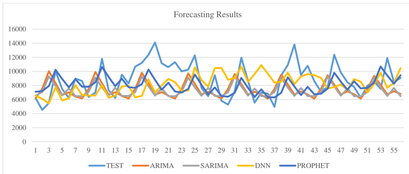
Figure 6. Forecasting outcomes for ATM 103
