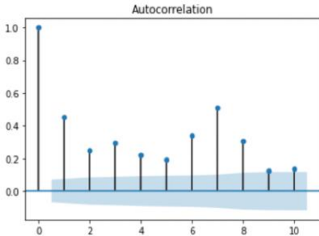
Figure 4. ACF values of the first ATM
