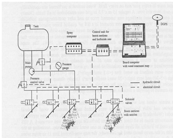
Figure 10. Precision spraying equipment for variable rate herbicide application (Gerhards et al, 1999).
